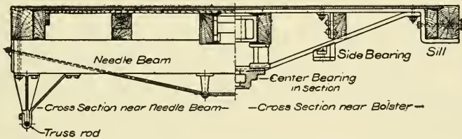
Fig. 4. Cross-Section of Underframe Showing Needle-Beam and Bolster
